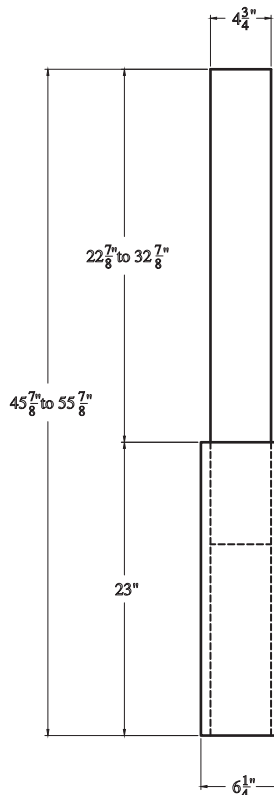
BN4091 6-1/4" x 45-7/8" to 55-7/8" Adjustable height fixed top block and loose mounting block O, MP, ALD, PL
