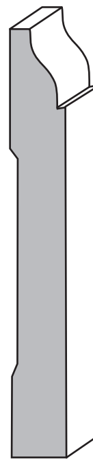
6343 7/16" x 3-1/4" MP, O, PRFJT
