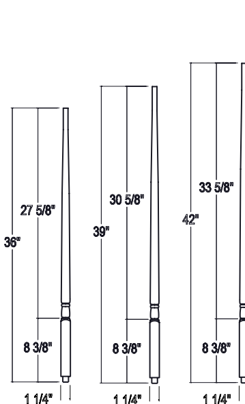
5015-5L 1-1/4" Square 36", 39", 42" O, PR
