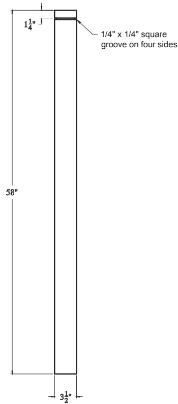
4001S 3-1/2" Square Angle ALD, PL
