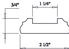
6045 w/6050 1-1/4" Plow 3/4" x 2-1/2" O, MP, PL, ALD w/6000F
