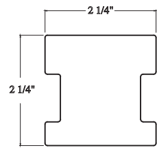
9200 2-1/4" x 2-1/4" ALD, PL
