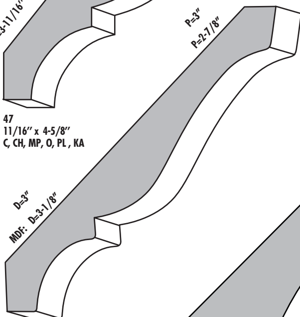
48 9/16" x 4-1/4" PRFJT, P
