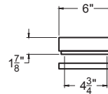
BN475FT-Cap Contemporary cap with 3/8" moulding 5/8" square moulding for base
