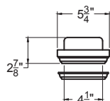
BN425HH-Cap 4091 style cap with moulding for cap and neck
