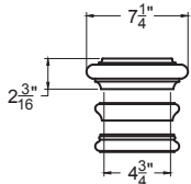
BN47592-Cap 4092 style cap with 4092U moulding for neck and base
