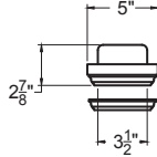
BN350HH-Cap 4091 style cap with moulding for cap and neck
