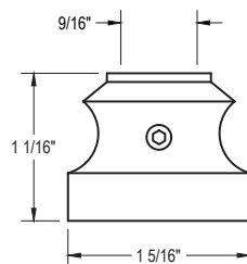
ALUM-LM-06 Alum. tall flat shoe w/ set screw for 1/2" Square- Pacific Collection SB
