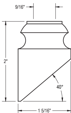
ALUM-LPSH-02 Alum. tall pitched shoe w/ set screw for 1/2" Square- Pacific Collection SB
