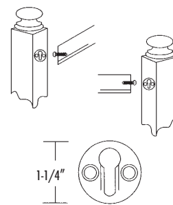
MiniLOCK FU-6287 Base plate is hardened steel, includes screws 2 per card
