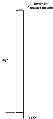
4000E 3-1/2" Square Starting O, MP, PL
