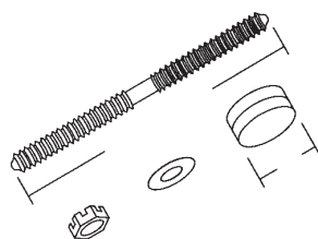
RailBOLT with Plug 2/PK-6288 0
