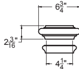
BN42592-Cap 4092 style cap with 4092U moulding for neck
