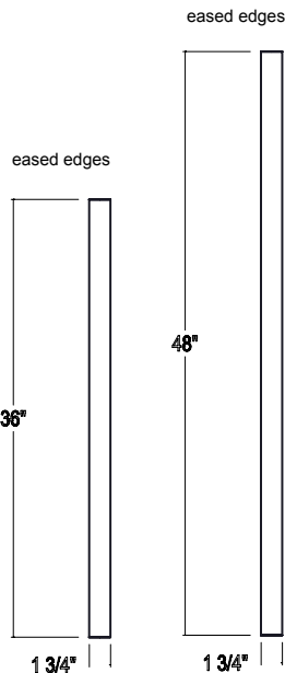
5360E 1-3/4" Square 36", 48" O, MP, PR
