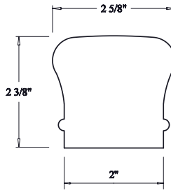
6210 2-3/8" x 2-5/8" O, MP, ALD, PL
