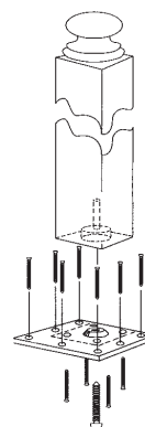
EZLOCK FU-6282 Base plate is hardened steel: 4-5/8" x 4-5/8" x 3/16" 13 screws included
