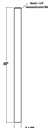
4001E 3-1/2" Square Landing O, MP, ALD, PL
