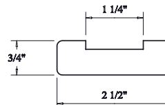
6000 w/6000F 1-1/4" Plow 3/4" x 2-1/2" O, MP, PL, ALD
