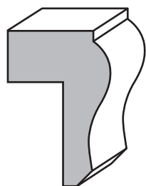
0612 3/4" x 1-1/8" MP, O, P
