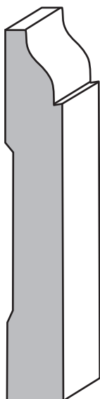
634 7/16" x 2-3/4" CH, MP, O, PL, KA, P
