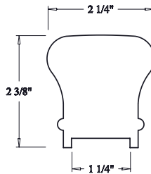
6010P w/6050 1-1/4" Plow 2-3/8" x 2-1/4" O, MP, PL w/6050 ALD w/6000F
