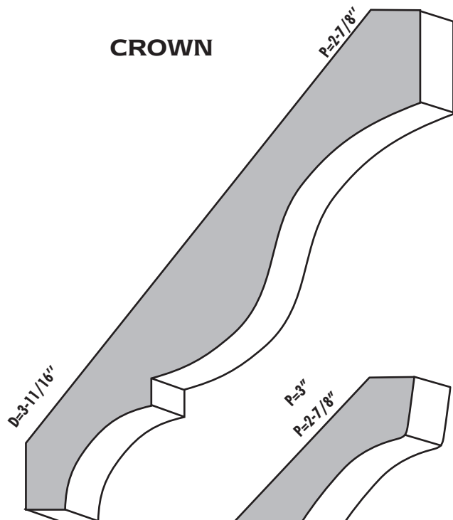
47 1 1/16" x 4-5/8" C, CH, MP, O, PL, KA
