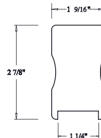
6206P w/6000F 1-1/4" Plow 2-7/8" x 1-9/16" O, MP
