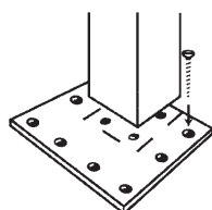
181 Newel Plate 3/16" x 5" x 6" Includes Screws
