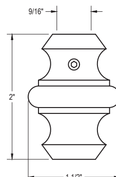
ALUM-LAK01 Adjustable Knuckle w/ set screw for 1/2" Square Bar SB
